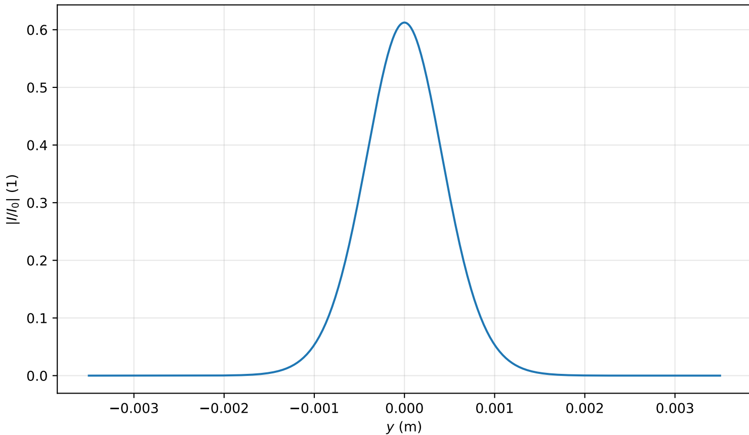
Intensity profile I(x=0, y, z=2.149)/I_0 , P_{in}=0.3P_{cr} , artificial time
